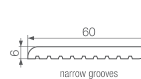
composite finishing strip dimensions (mm)
