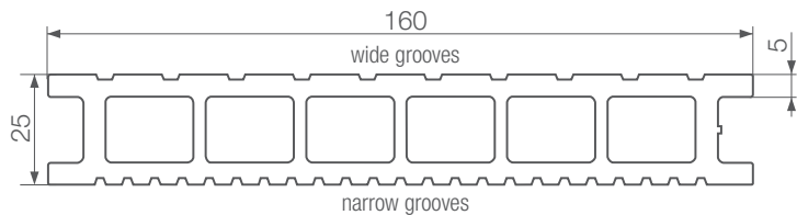
board dimensions (mm)
