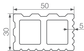
joist dimensions (mm)
