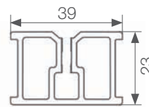
aluminum joist dimensions (mm)
