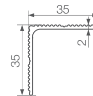
finishing strip (anodized aluminium) dimensions (mm)
