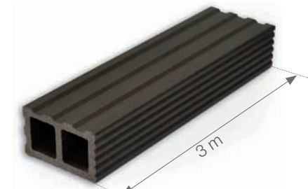
joist
